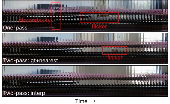
Figure 7. Temporal quality. Vertical slices of a rendered novel camera path on the BONSAI scene from Mip-NeRF360 [41] illustrate the temporal quality across adjacent viewpoints. One-pass or gt + nearest procedural sampling results in notable flickering, whereas interp procedural sampling ensures temporally smooth rendering.
