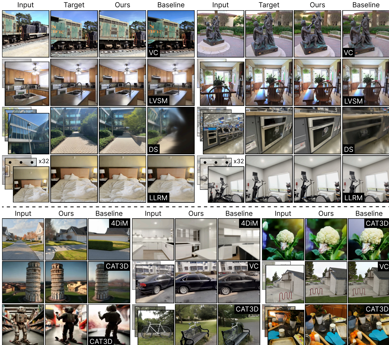
Figure 6. SOTA comparison on set NVS (top) and trajectory NVS (bottom) across varying numbers of input views. We compare with open-source approaches—ViewCrafter [9] (VC) and DepthSplat [44] (DS)—as well as proprietary ones including LVSM [11], LongLRM [17] (LLRM), 4DiM [12], and CAT3D [8]. When the input comprises multiple views, we arrange them so that the view closest to the target is placed at the top of each set.
